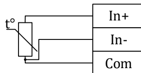
RTD sensors (3-wire)
