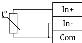
RTD sensors (2-wire)
